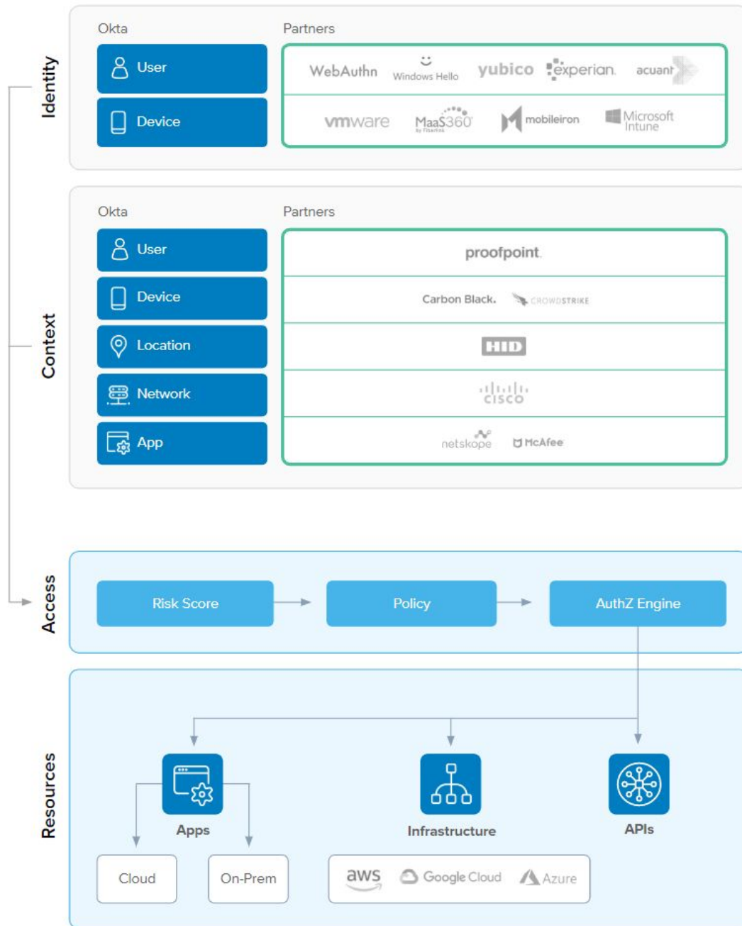
Zero Trust Reference Architecture
