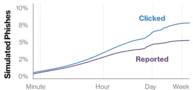
Click, reporting rate in public simulated phishes over time
